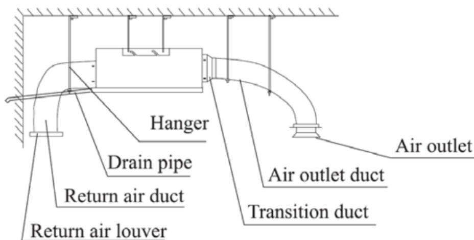
Typical duct arrangement
